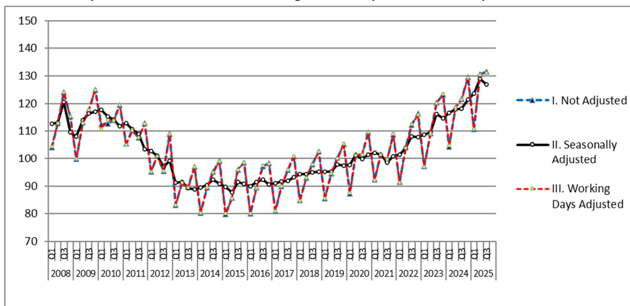
Graph 1: Evolution of the Index of Wages Cost: 1 st quarter 2008 – 3 rd quarter 2025
